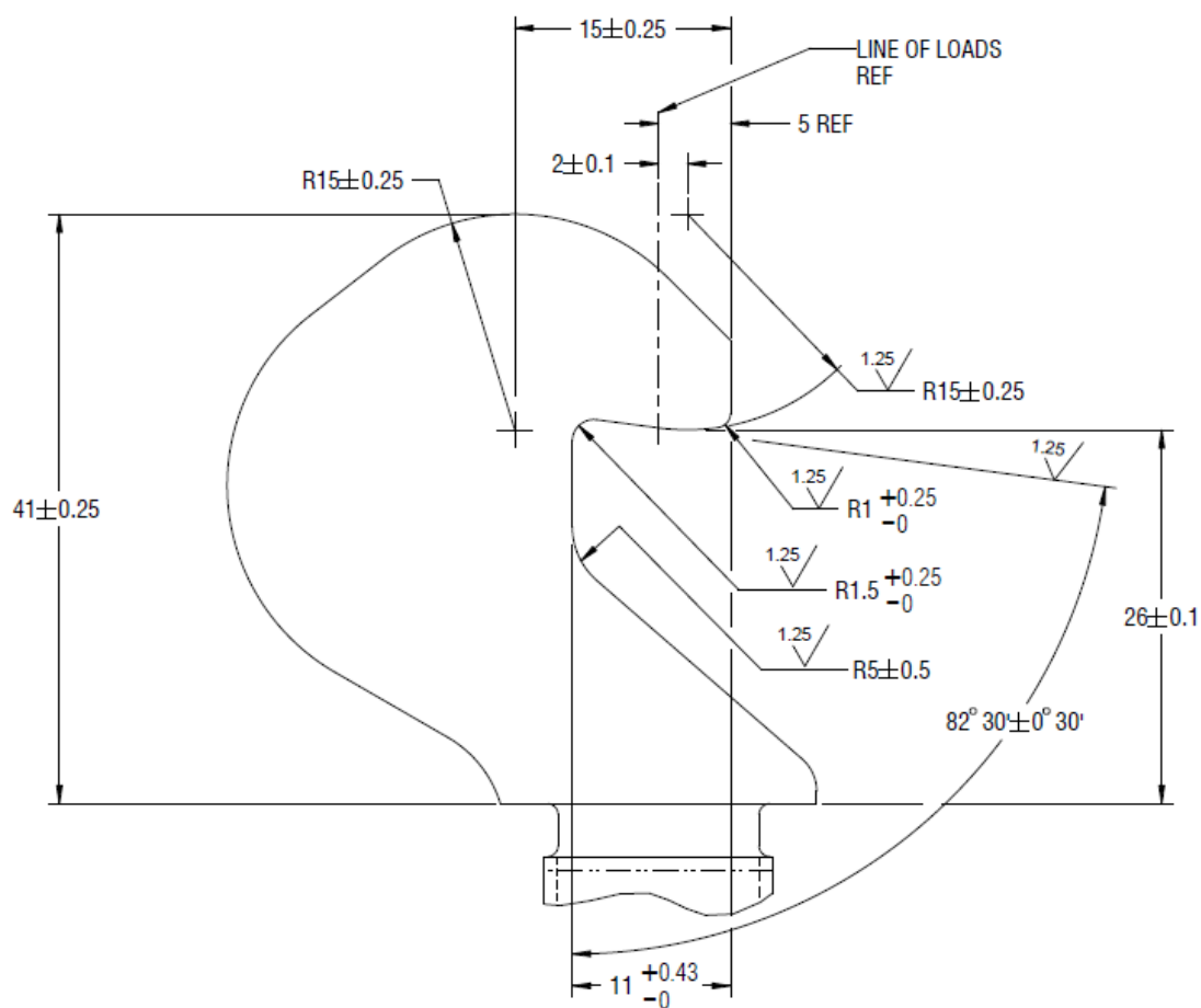
FIGURE 3.2.3.4-6 PASSIVE HOOK DETAIL VIEW
