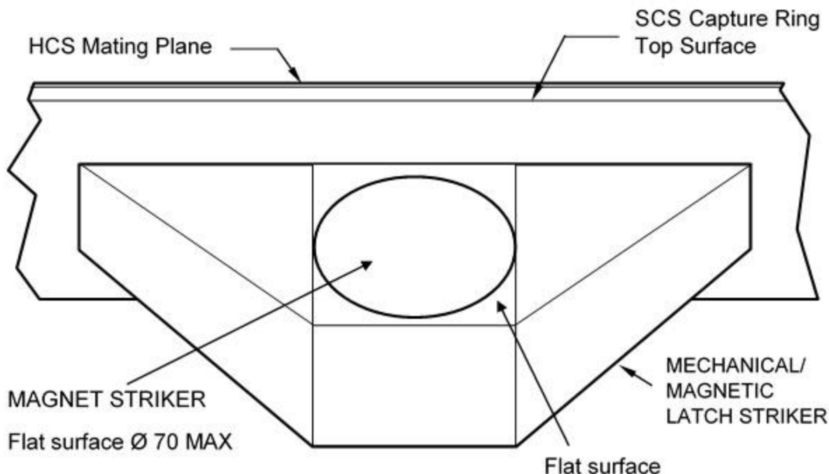
FIGURE E.1.0-2 RADIAL VIEW
