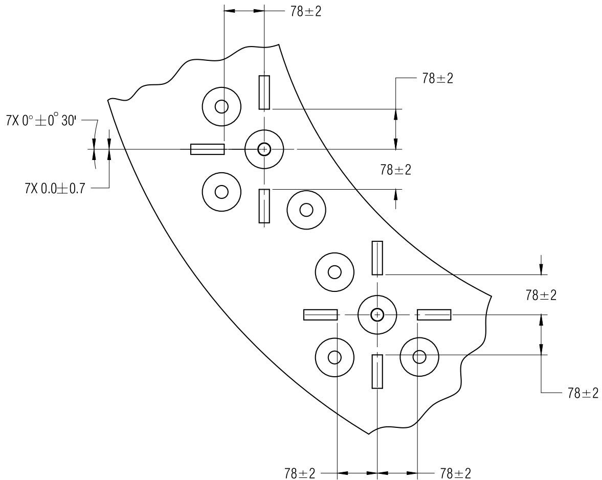
FIGURE 3.5.3.18-1 PVT CROSSHAIR LOCATIONS IN PDT (A) AND PDT (B) COORDINATES
