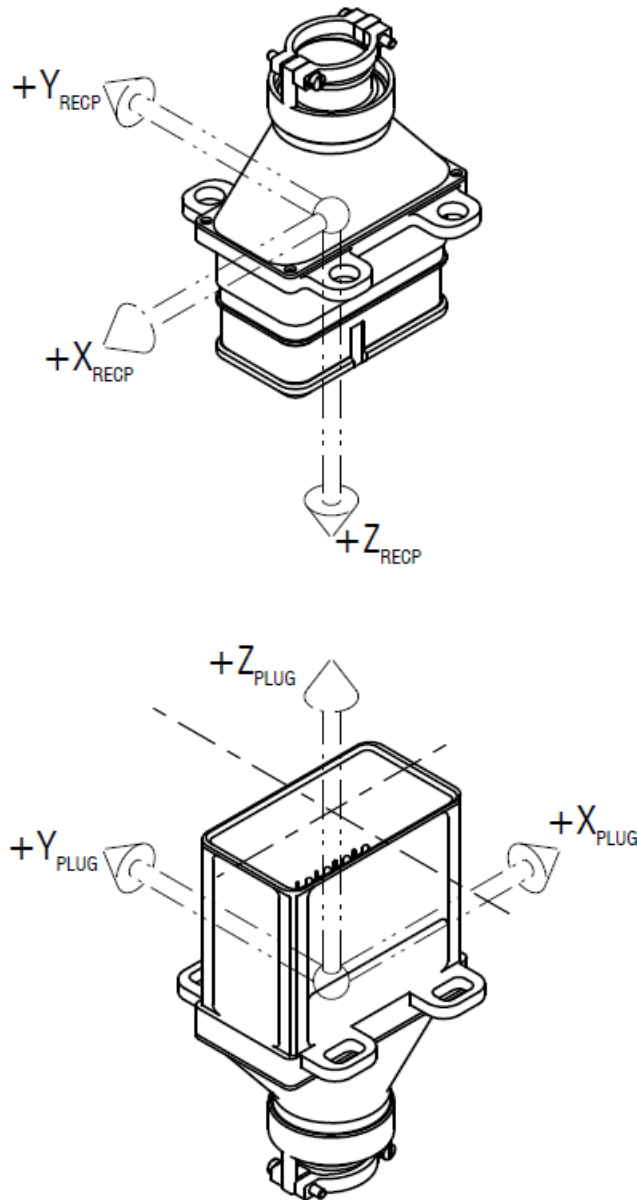
FIGURE 3.4.1.3-1 PDU CONNECTOR LOCAL COORDINATE SYSTEM DEFINITION
