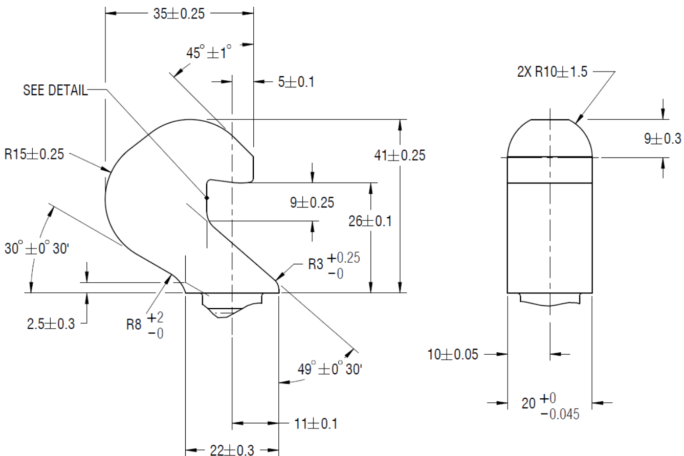
FIGURE 3.2.3.4-5 PASSIVE HOOK
