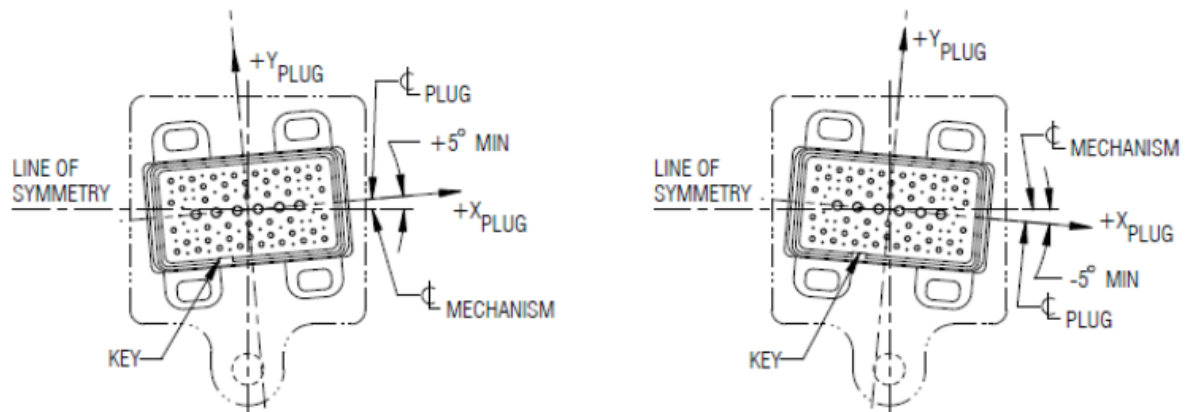
FIGURE 3.4.1.5.1.2-1 PLUG ROTATIONAL COMPLIANCE ABOUT THE Z AXIS
