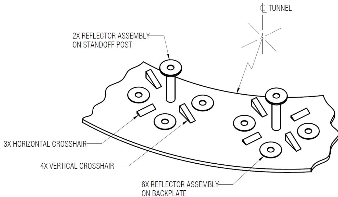
FIGURE 3.5.3-1 PERIPHERAL DOCKING TARGET
